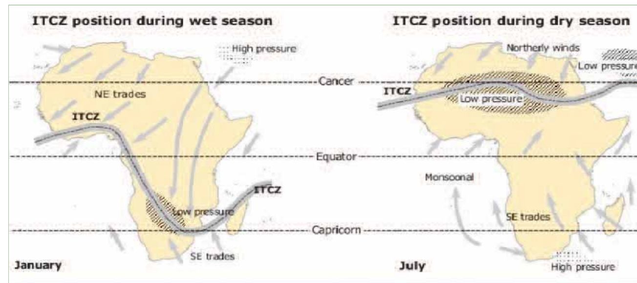
Figure 4. 3 ITCZ and Rain in Africa
