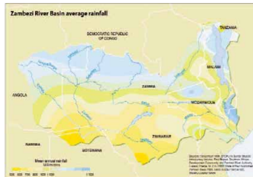
Figure 4. 4 Average rainfall pattern
