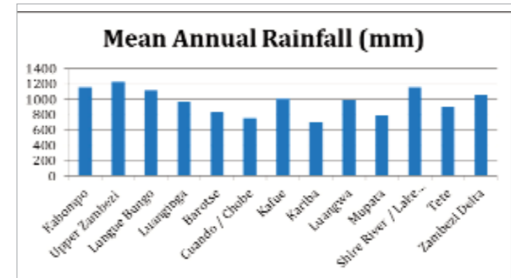
Figure 4.5 Average rainfall pattern for Major sub-basins
