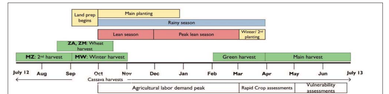
Figure 5. 1 Agricultural calendar in a typical year in Southern Africa
