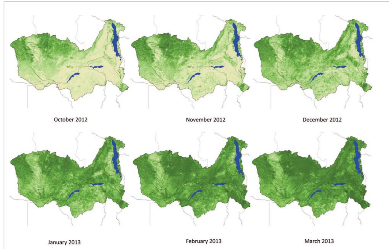
Figure 5.7 Vegetation Condition per month for 2012/2013 Agricultural Season
