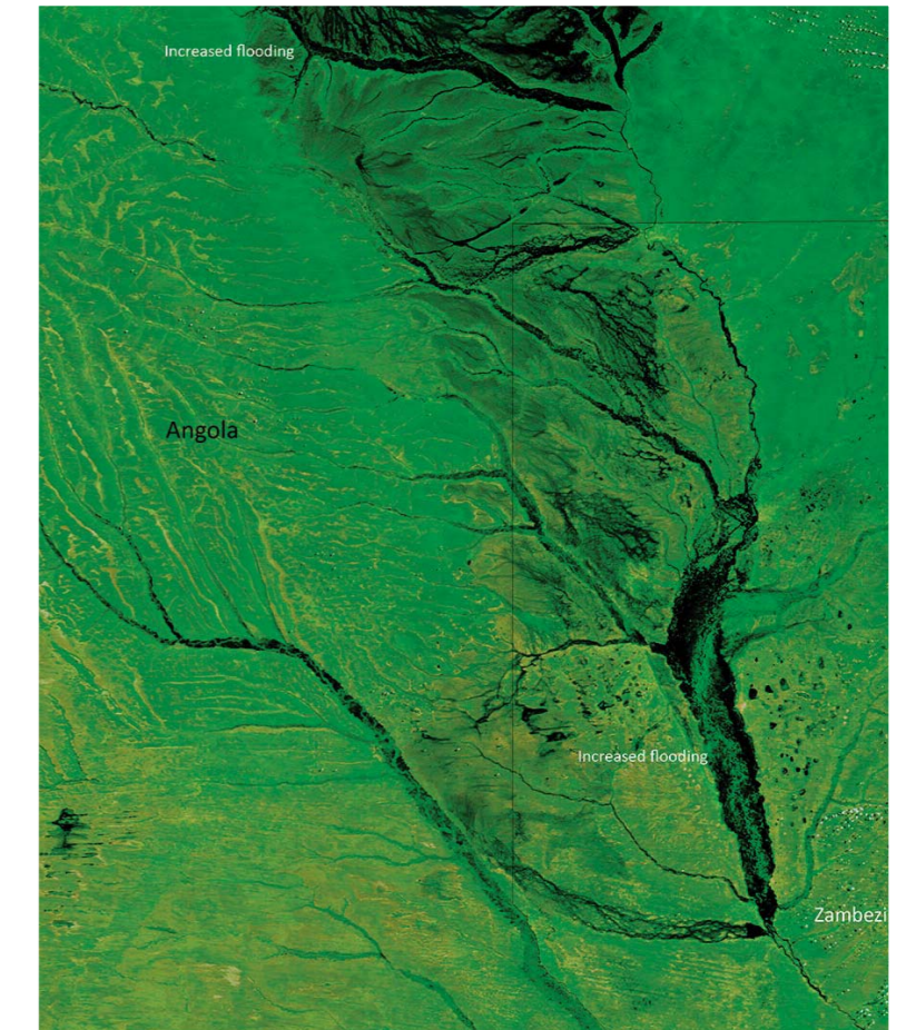
Figure 3.6 b Satellite image of the “swollen” Zambezi Floodplains under flooding
