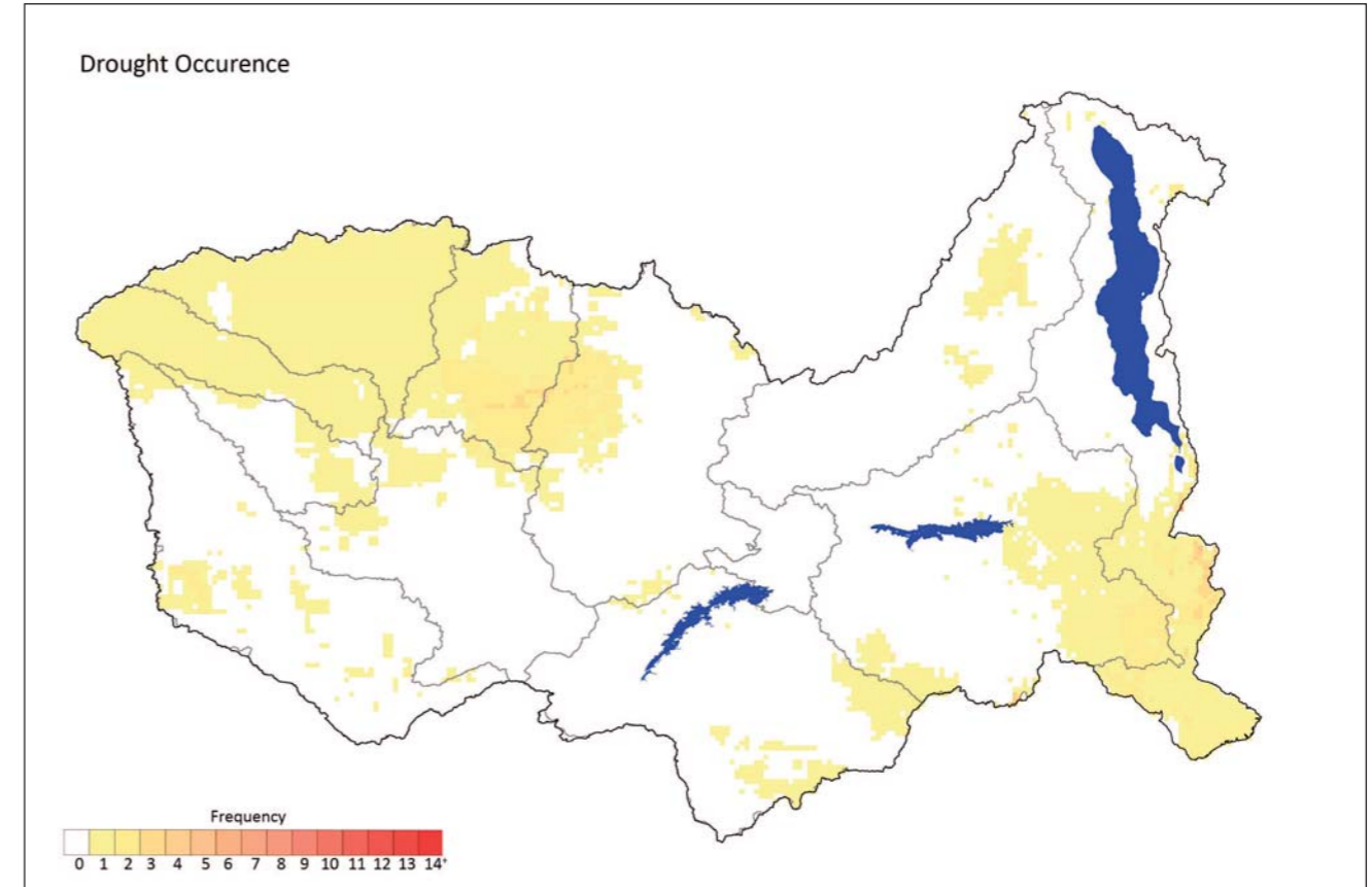
Figure 5.4 a Occurrence of Severe dry periods during the OND period over 18 years (1995 to 2013).
