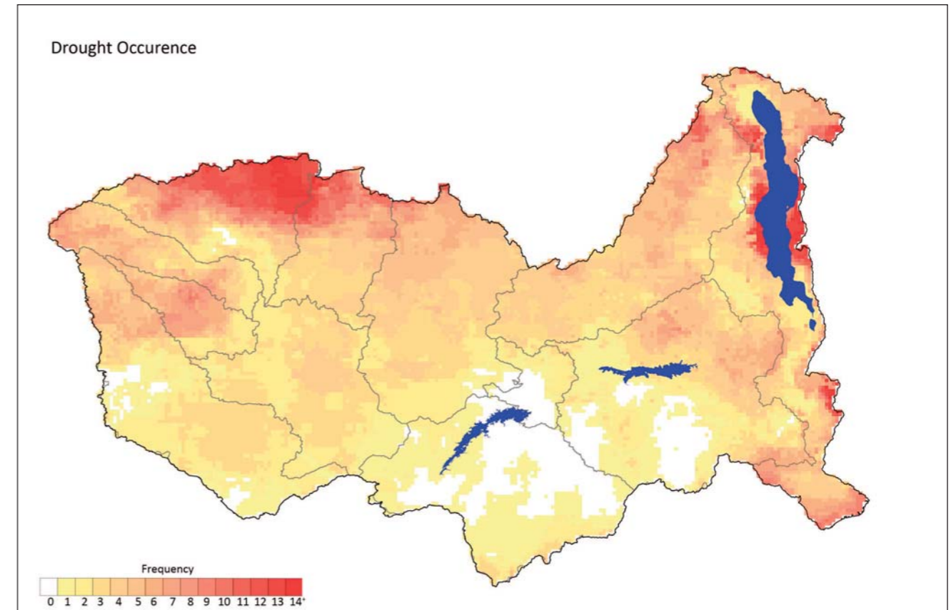
Figure 5.4 b Occurrence of Severe dry periods during the JFM period over 18 years (1995 to 2013).
