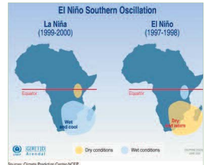
Figure 4. 1 El Niño and La Niña effects in Southern Africa
